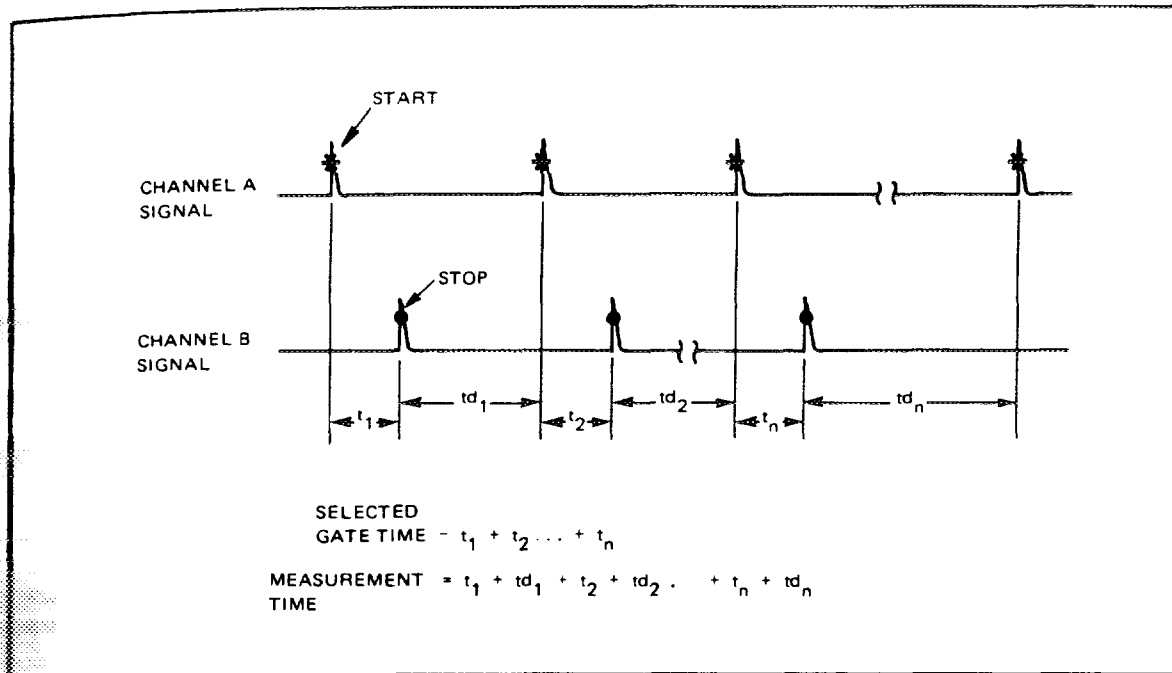
Figure 3-1. Measurement Time for Time Interval Average
