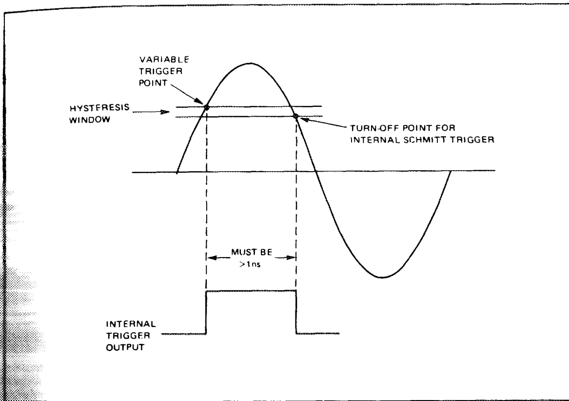
Figure 3-2. Internal Triggering
