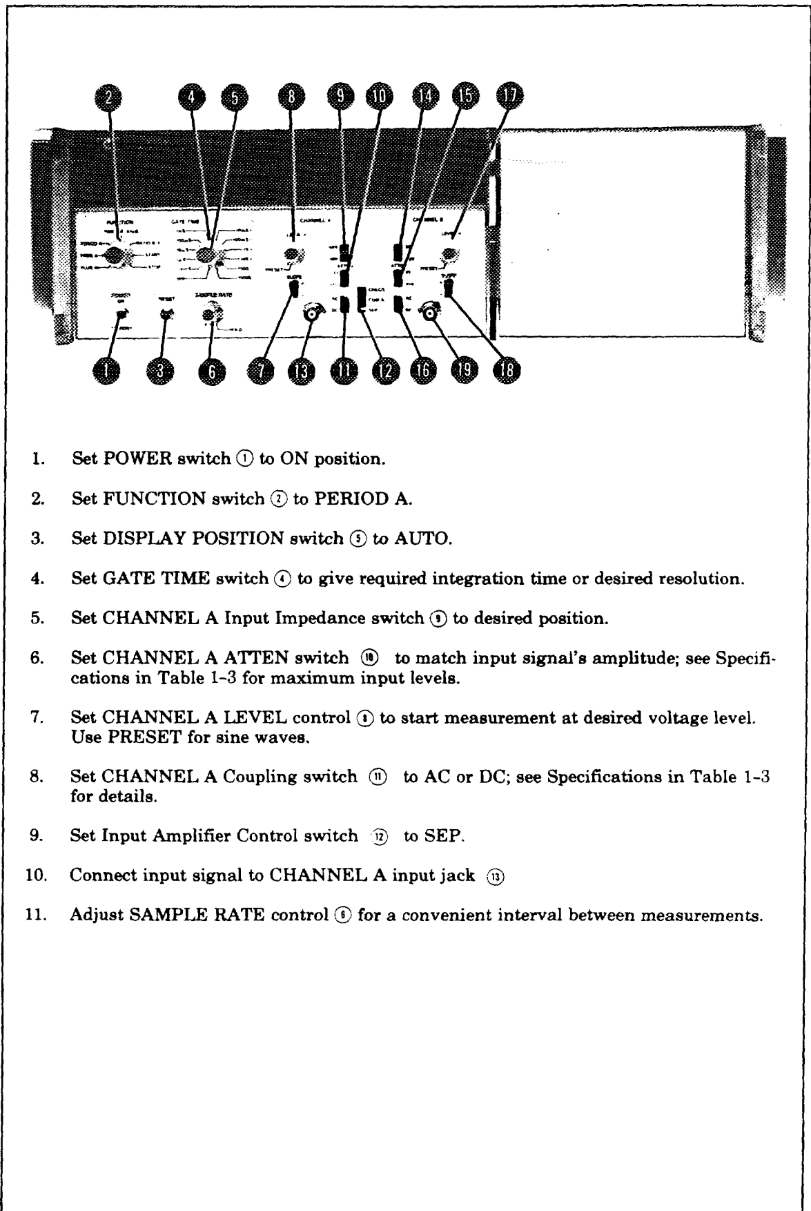
Figure 3-13. Period Measurements
