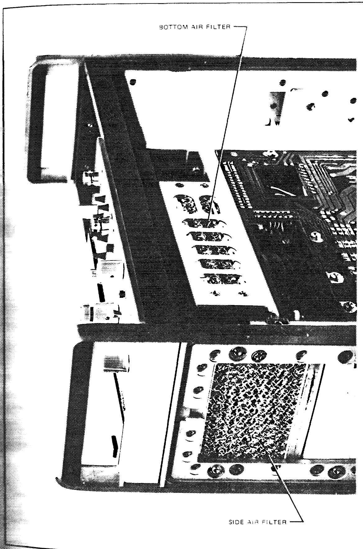
Figure 3-9. Location of Air Filters
