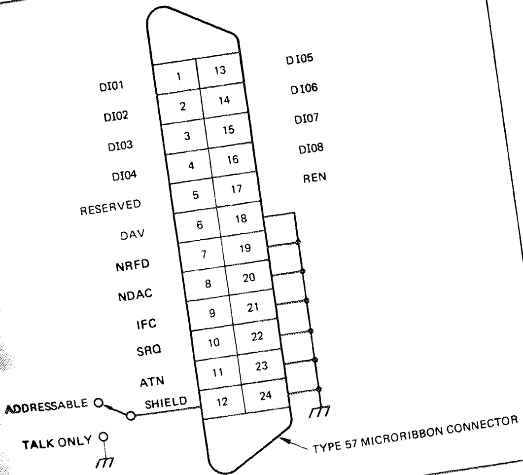
Figure 2-3. 5345A Digital Input/Output
