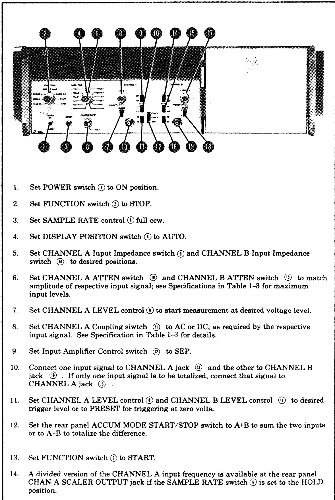
Figure 3-17. Totalize Measurements
