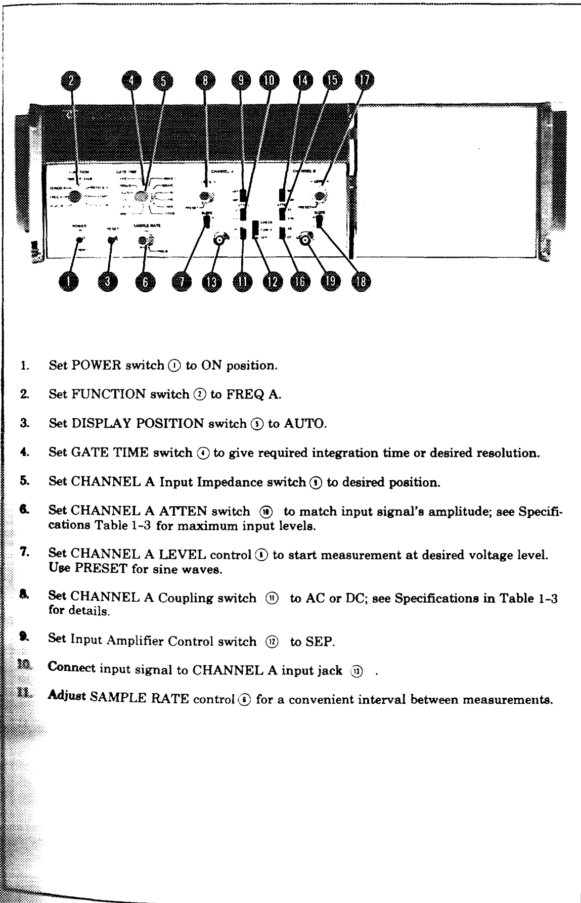
Figure 3-12. Frequency Measurements
