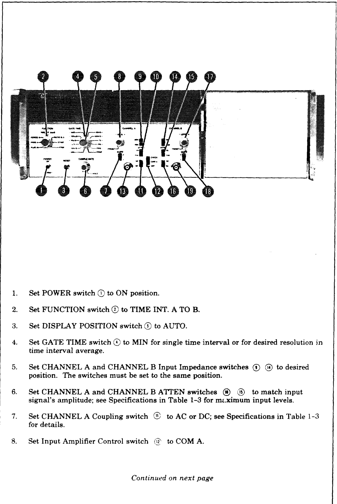
Figure 3-15. One Source Time Interval Measurements
