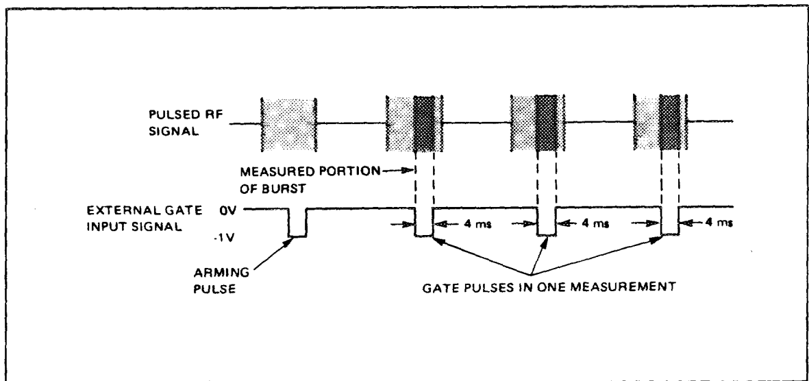
Figure 3-3. Multiple Gating
